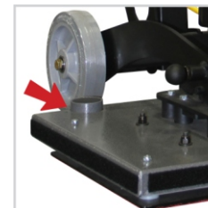
Frame is Built with Dual Vacuum Ports for Use on TH2814-V
